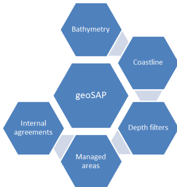
Figure 399. GeoSAP content.
